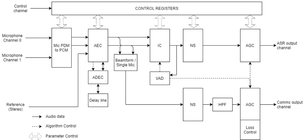
Fig. 3.1: The XVF3615 audio pipeline
