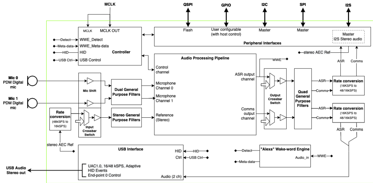
Fig. 3.4: XVF3615-UA-HYBRID System architecture
