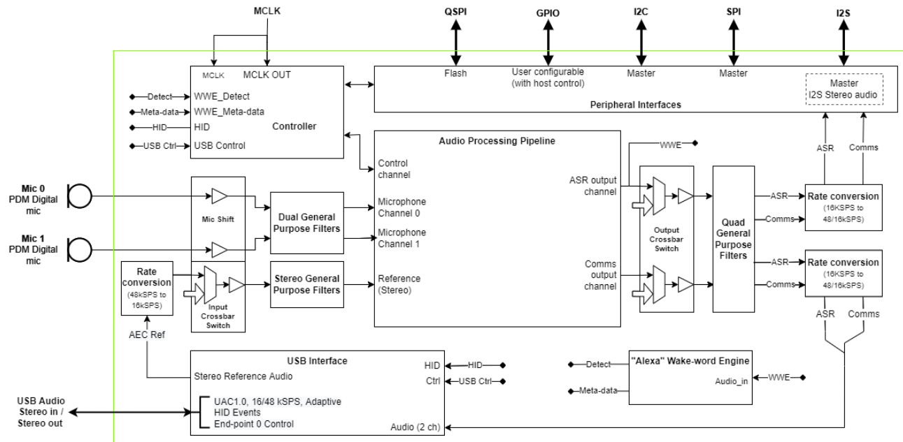
Fig. 3.3: XVF3615-UA System architecture
