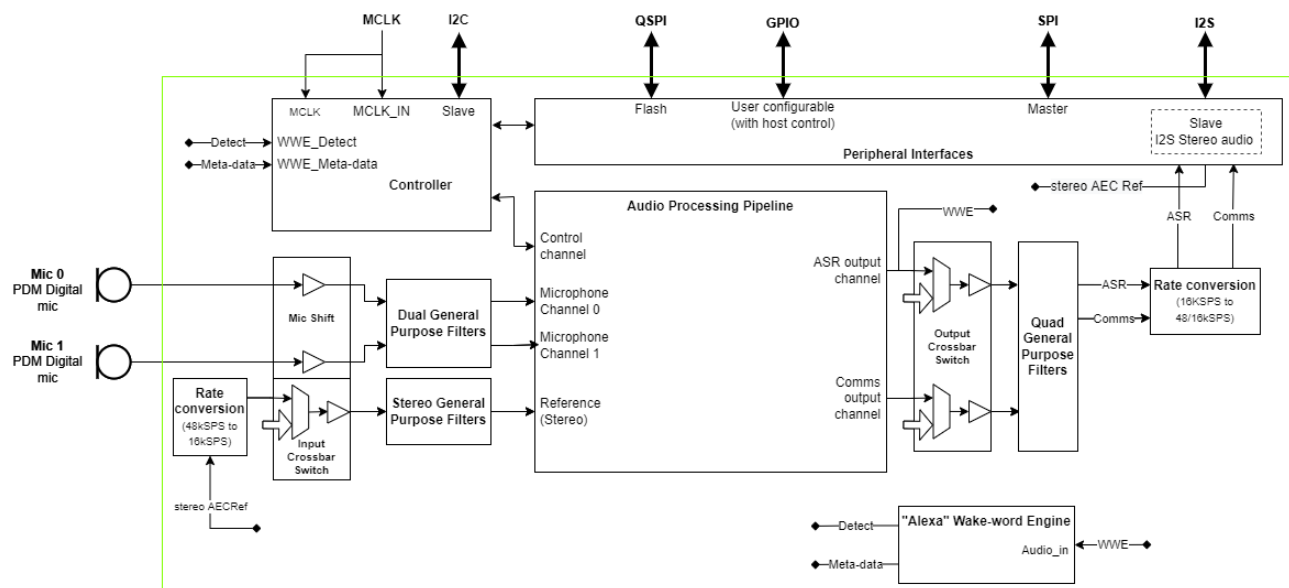
Fig. 3.2: XVF3615-INT System architecture
