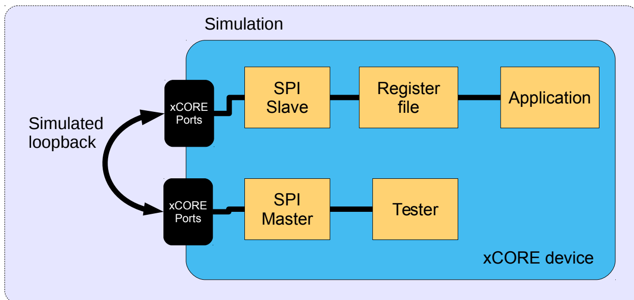
Figure 1: Block diagram of SPI slave application example
