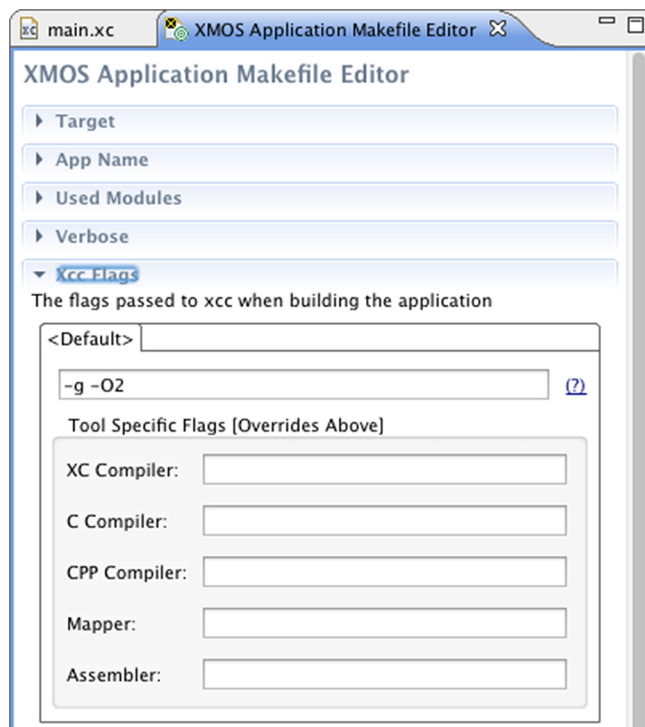
Figure 1: Makefile Editor
